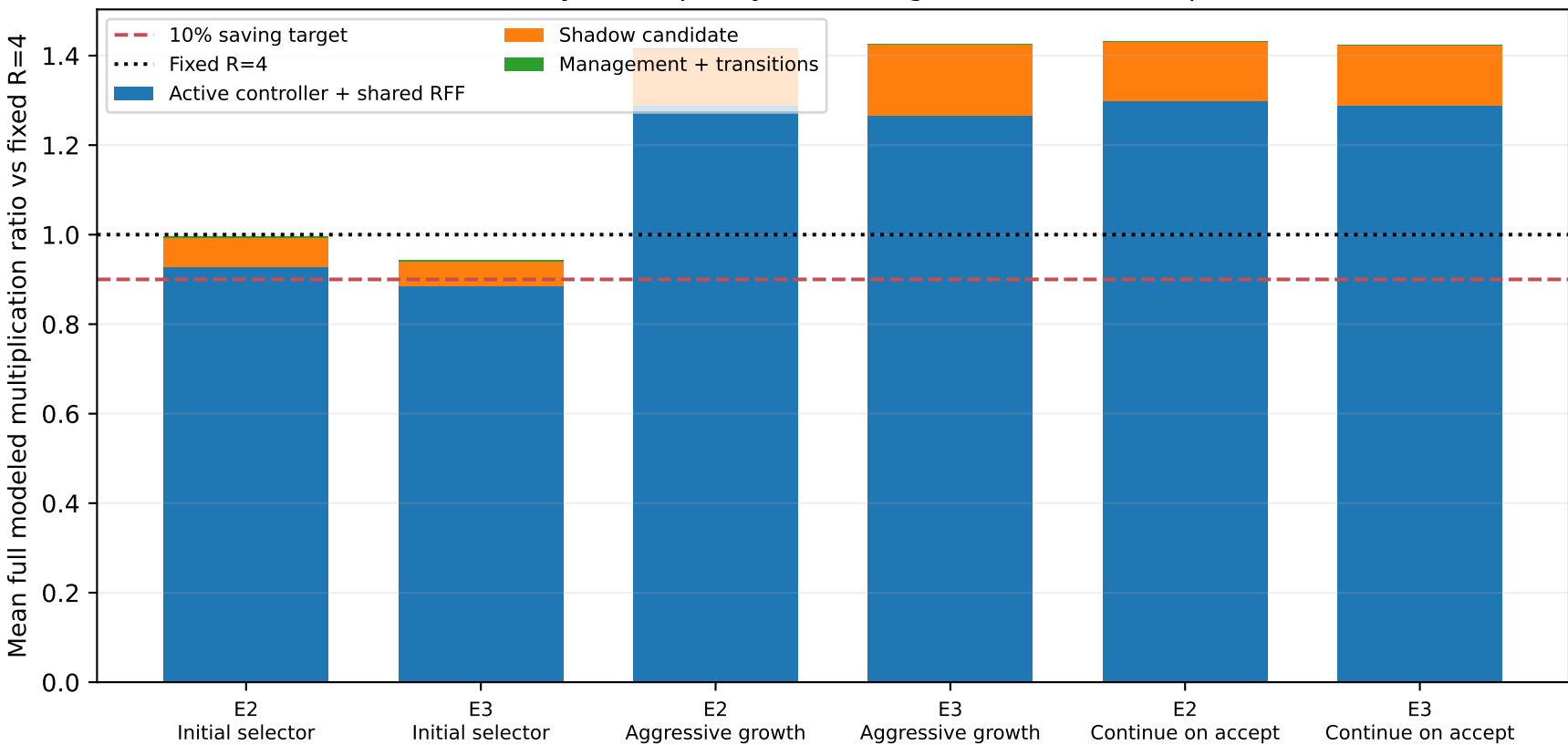
Nonstationary ANC: quality/cost design tradeoff (development)
