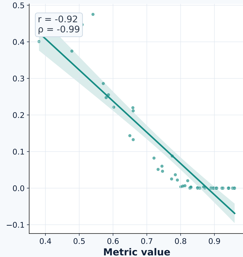
Pillai
