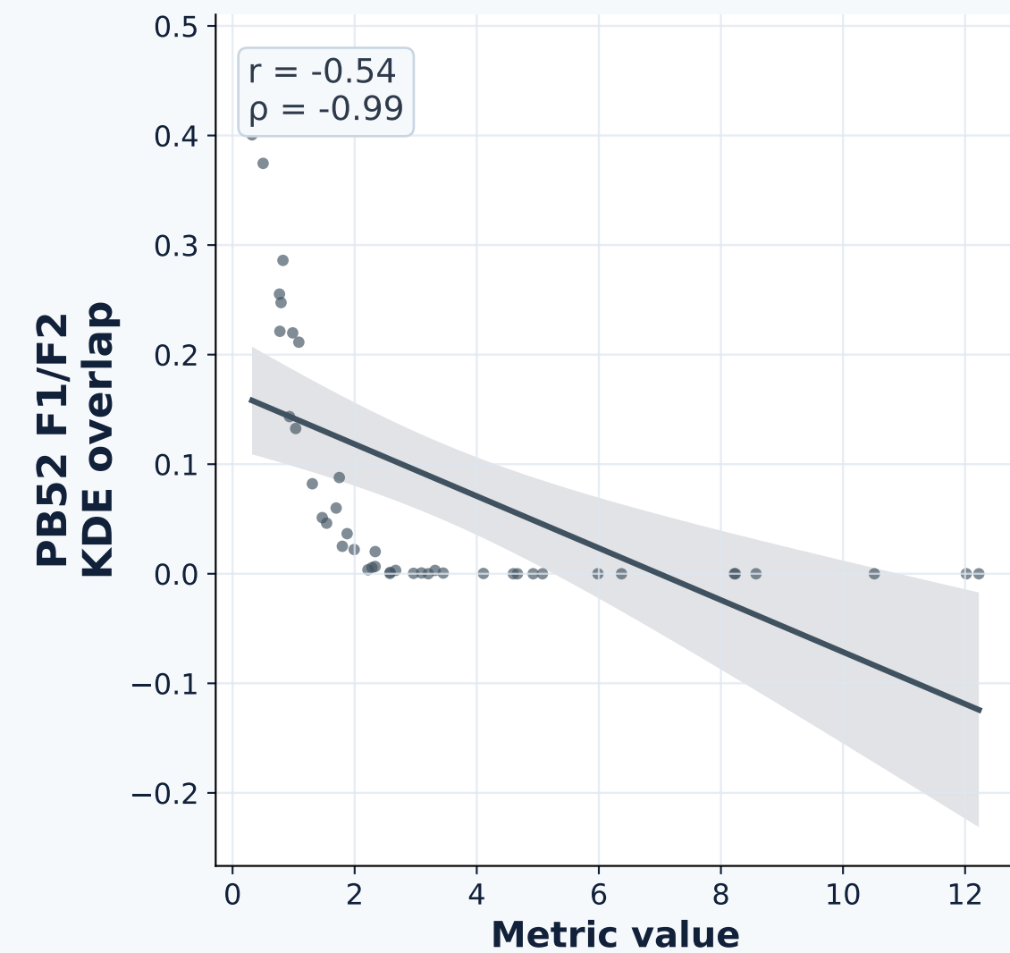
Bhatt. distance
