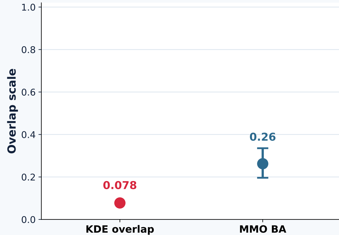
Overlap estimates
