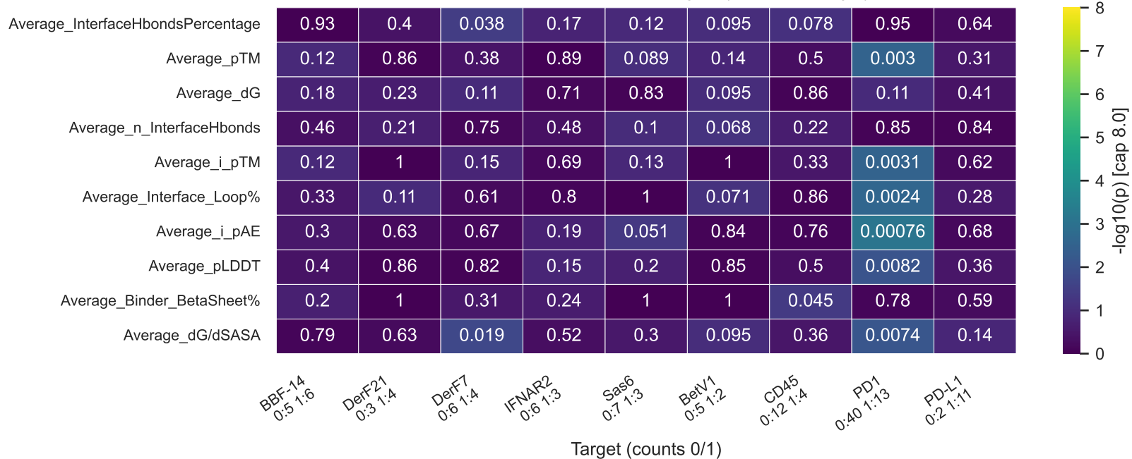
Shared top-10 metrics across targets (top-10 per target)
