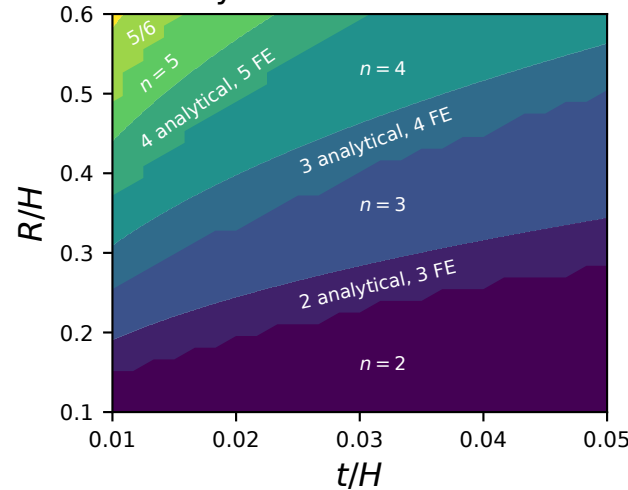
Analytical vs Linear Buckle
