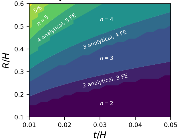
Analytical vs Linear Buckle
