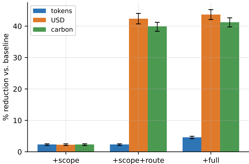
Multi-step ablation (SWE-rebench, 95% CI)
