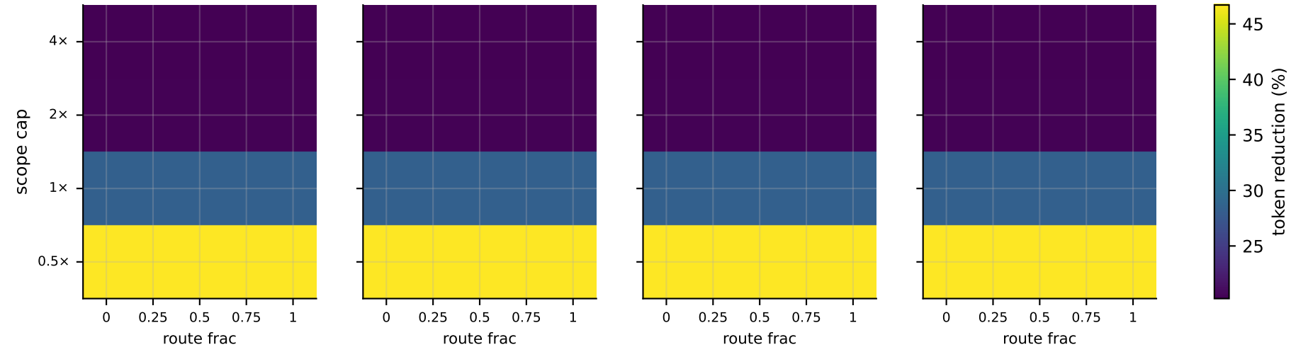
Token reduction over (scope cap \times route), per \delta
