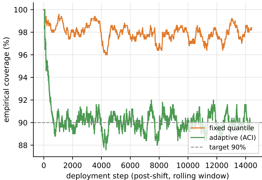
Coverage under distribution shift
