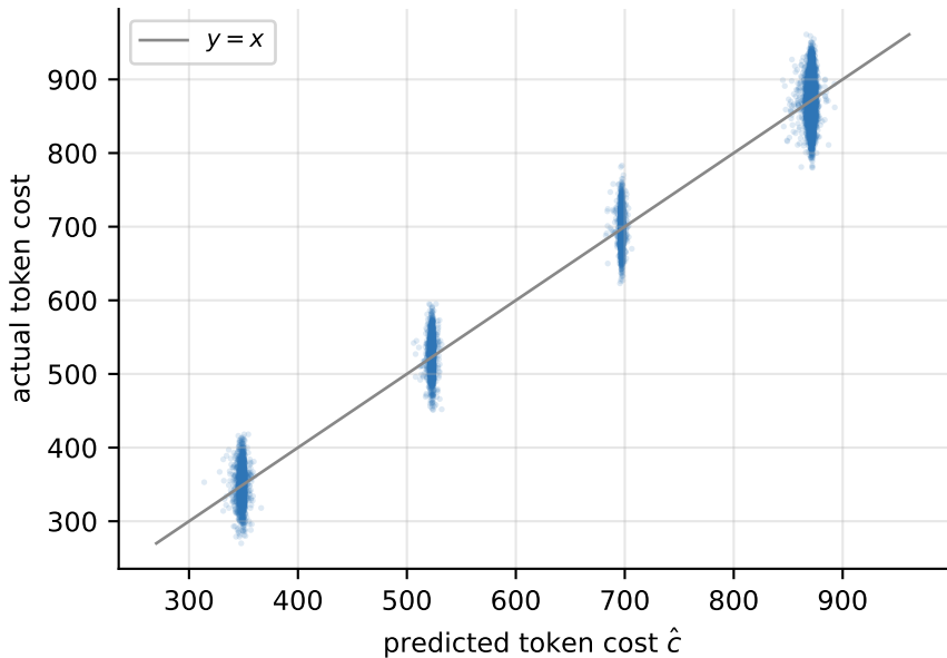
Forecast calibration ( R^2 = 0.980 , WAPE=2.6%)
