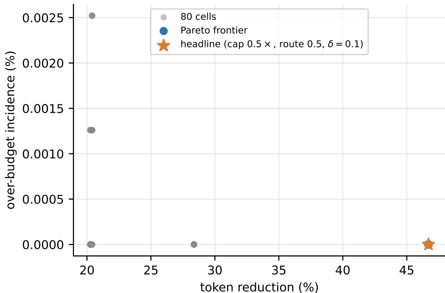
Joint sensitivity: 80 operating points
