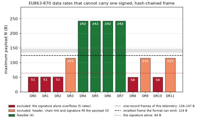
Fig. 2. Maximum payload of the twelve EU863-870 data rates against the smallest frame the lean format can emit and the frames this telemetry produces (64 B signature).
