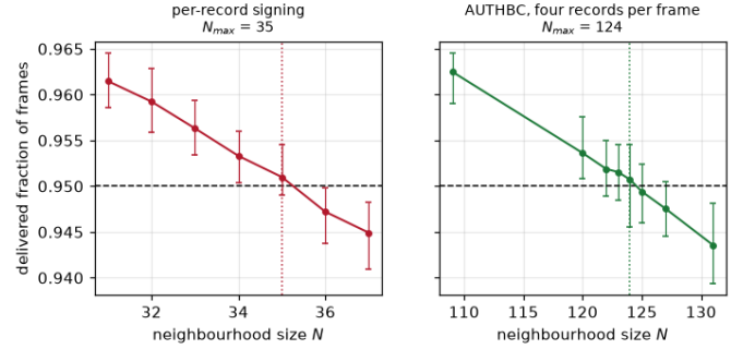
Fig. 3. Delivered fraction of frames against neighbourhood size in ns-3, lean format: baseline (row 5) and design (row 8). Mean of 30 runs; bars span the runs. N_{\max} is where a curve leaves the 0.95 line.
