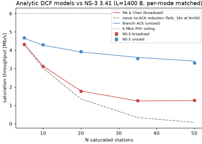
Fig. 3. Analytic DCF models vs. NS-3 3.41 saturation throughput. Unicast matches Bianchi within +0.6%/−2.9%; broadcast matches Ma and Chen [2] within 1.1%, while the naive reduction of the unicast model (dashed) fails by 16× at N=50 .
