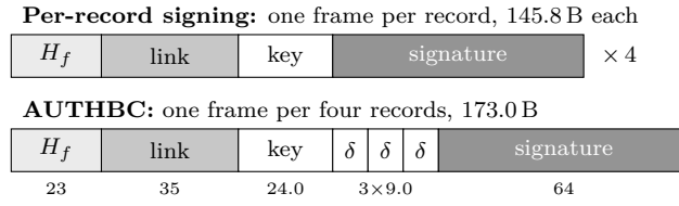
Figure 3.1: The lean frame, to scale (bytes below). Per-record signing repeats header, chain link and signature with every record; the design carries them once per four records, and the three records after the first are coded as differences ( \delta ).
