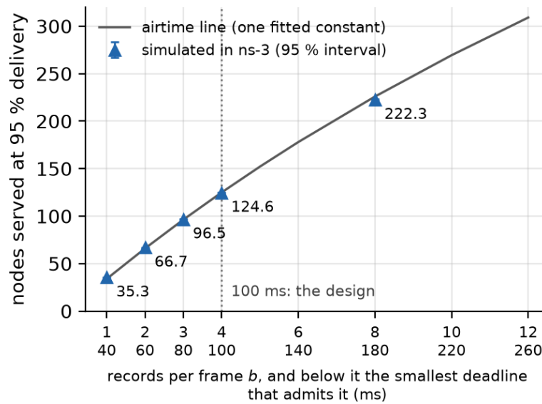
Figure 8.3: The neighbourhood the lean design serves at 50 records/s, by batch size and the smallest deadline that admits it: the five simulated crossings of 0.95 delivery (95% intervals, smaller than the markers) and the airtime line through the batch sizes that were not simulated. At 40 ms the batch is one record and nothing is gained.
