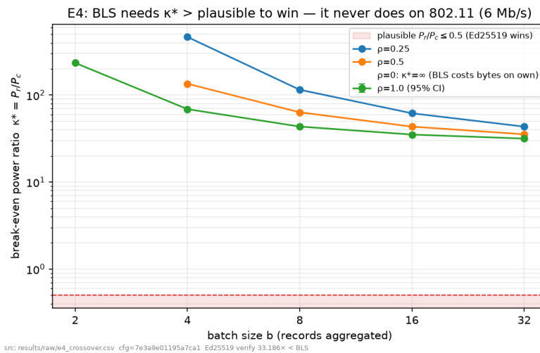
Figure 8.2: The scheme crossover. BLS becomes worthwhile only in the cross-signer regime.
