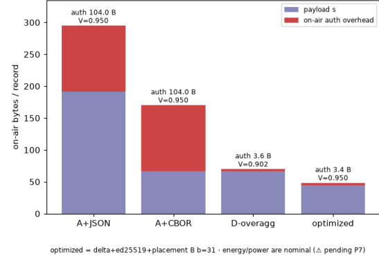
E5 co-design (T5): optimized cuts auth bytes 96.8% vs A+CBOR at V \geq 0.95 , p=0.05 [PASS]
