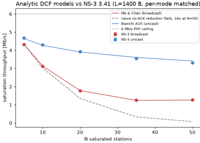
Fig. 3. Analytic DCF models vs. NS-3 3.41 saturation throughput. Unicast matches Bianchi within \pm 0.6\% – 2.9\% ; broadcast matches Ma and Chen [2] within 1.1\% , while the naive reduction of the unicast model (dashed) fails by 16\times at N=50 .
