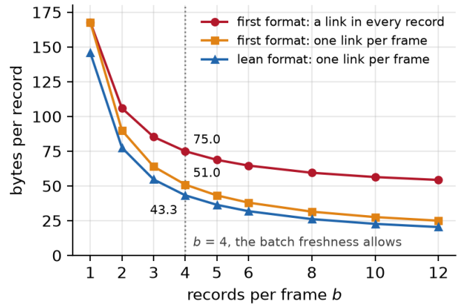
Fig. 3. Bytes per record against batch size, by where the chain link sits (delta records throughout). First-format curves are sums of measured parts; lean frames are emitted.
