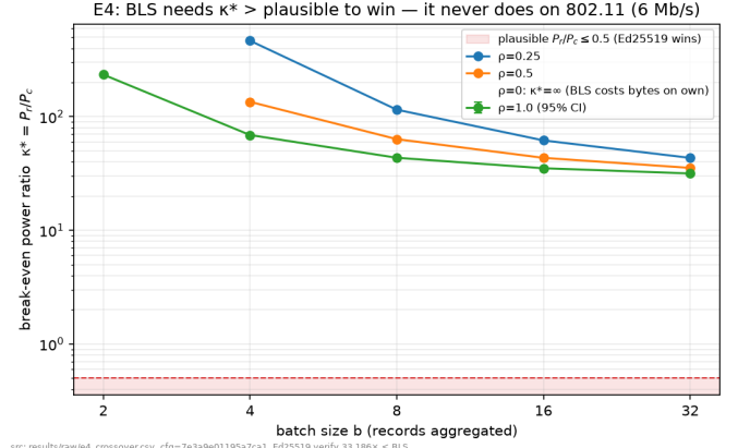
Fig. 2. E4: break-even power ratio \kappa^*(b) per relay fraction. Every curve sits far above the plausible band ( \kappa \leq 0.5 ), so Ed25519 wins on 802.11; the p=0 curve is \infty (BLS costs bytes on own traffic).
