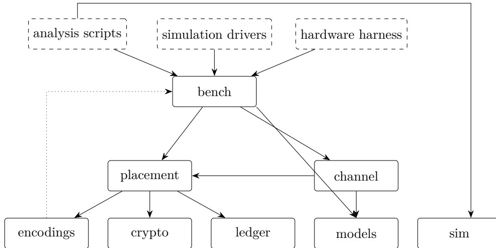
Figure 5.1: The packages of the library (solid) and what runs them (dashed). An arrow points from a package to one it uses; arrows that follow from others are omitted. The dotted arrow is the one upward reference: the encoders take the record type from the telemetry generator.
