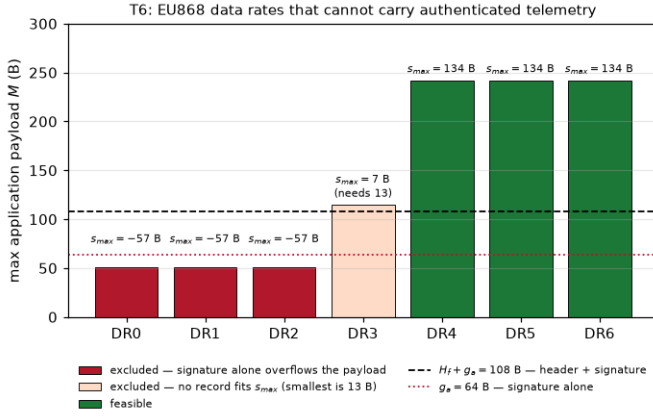
Fig. 6. Boundary 1. The payload-exclusion tiers across EU868 data rates at H_f=44 B measured and g_a=64 B. DR0–2 are excluded by the signature alone — no header design, encoding, batching or chaining reaches them — and DR3 misses on the record by six bytes. Only DR4–6 admit per-frame-verifiable telemetry. The boundary is arithmetic, so unlike the capacity results it does not move with the channel model.
