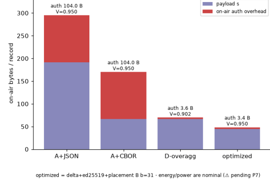
E5 co-design (T5): optimized cuts auth bytes 96.8% vs A+CBOR at V \geq 0.95, p=0.05 [PASS]
