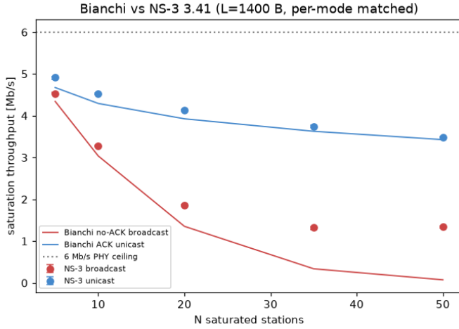
Fig. 3. Bianchi vs. NS-3 3.41 saturation throughput. Unicast matches within \pm 5\% ; broadcast is capture-limited above the no-ACK analytic lower bound.
