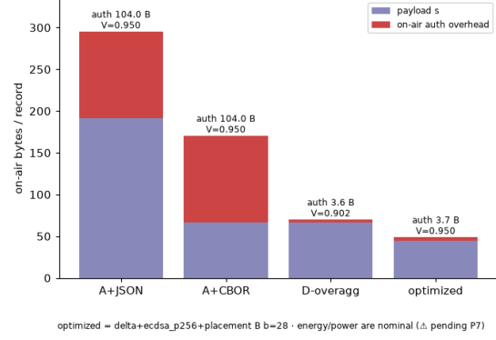
E5 co-design (T5): optimized cuts auth bytes 96.4% vs A+CBOR at V \geq 0.95 , p=0.05 [PASS]
