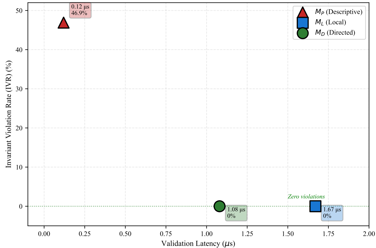
Latency-Compliance Trade-off ( n = 5, k = 3 )
