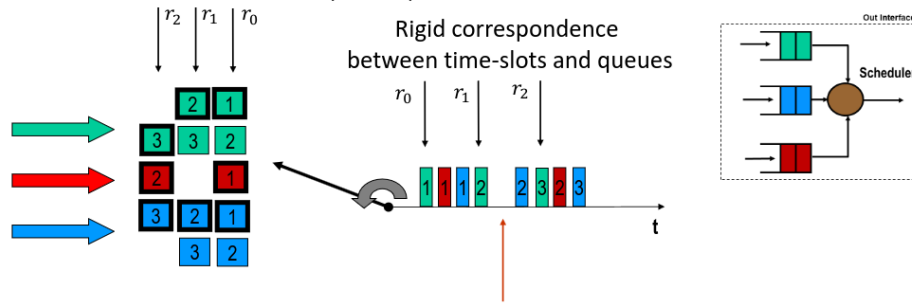
Figure 5.2: Time division multiplexing
