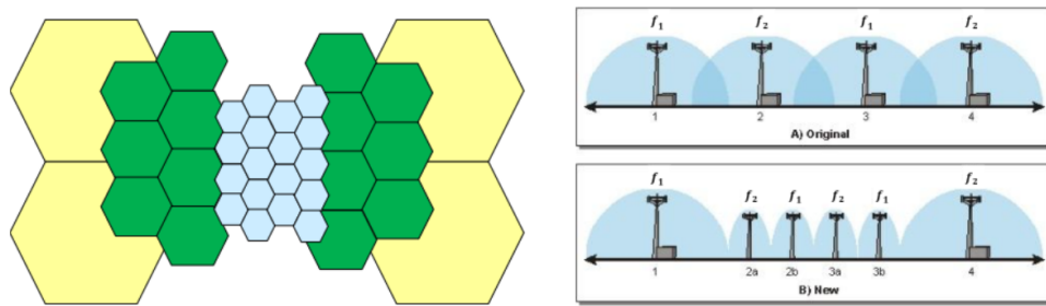
Figure 8.14: Cell splitting
