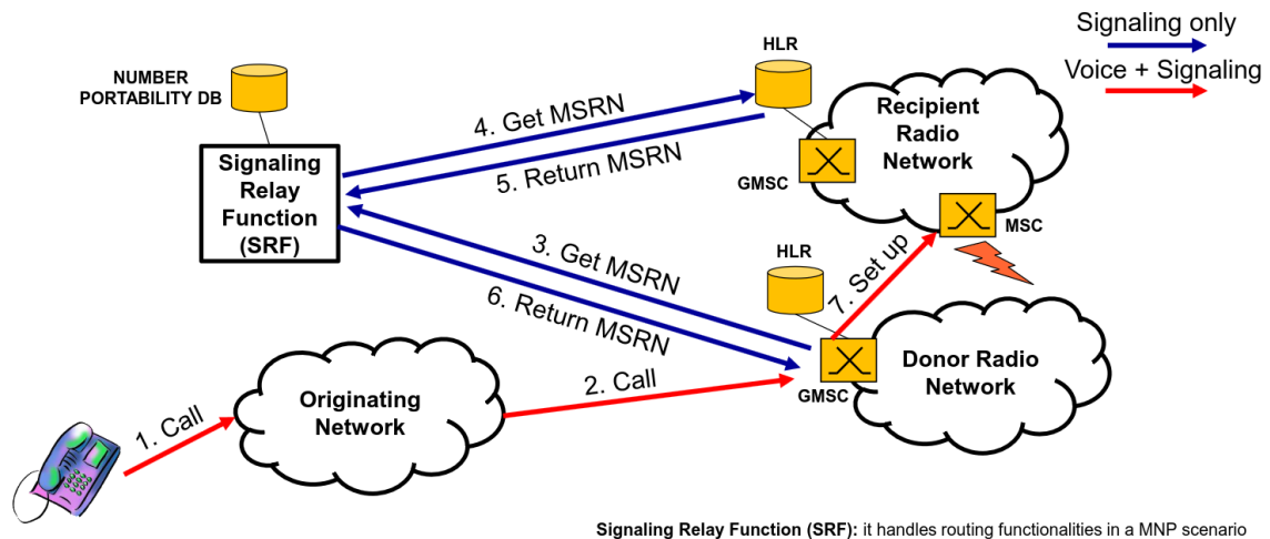
Figure 9.13: Mobile number portability
