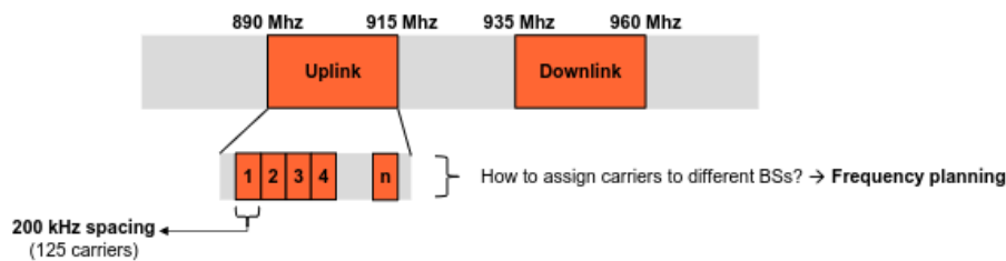
Figure 8.7: Frequency planning
