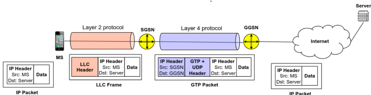
Figure 9.17: Tunneling in GPRS/EDGE
