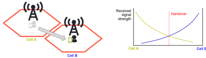
Figure 8.6: Handover
