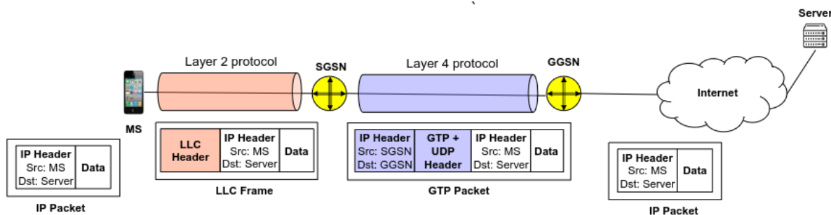
Figure 9.14: Tunneling in GPRS/EDGE
