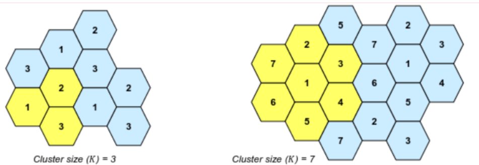
Figure 8.10: Frequency reuse
