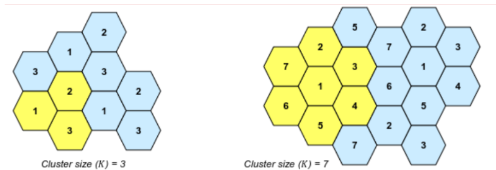
Figure 8.10: Frequency reuse
