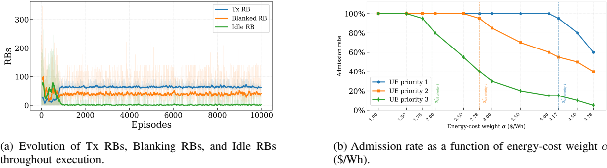
Fig. 6: Admission rate versus the energy-cost weight \alpha . Dashed lines denote the break-even thresholds \alpha^* = H(y)/E(x, y, z) , showing that lower-priority UEs are rejected first.
