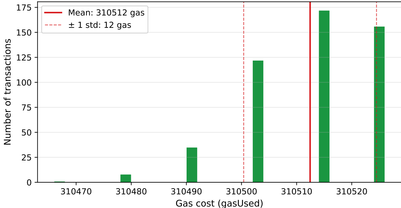
On-Chain ZKP Verification Gas Cost Distribution (n=494)
