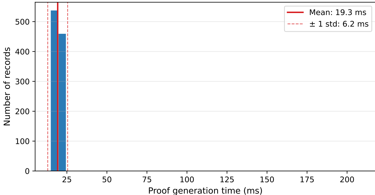
ZKP Proof Generation Time Distribution (n=1000)
