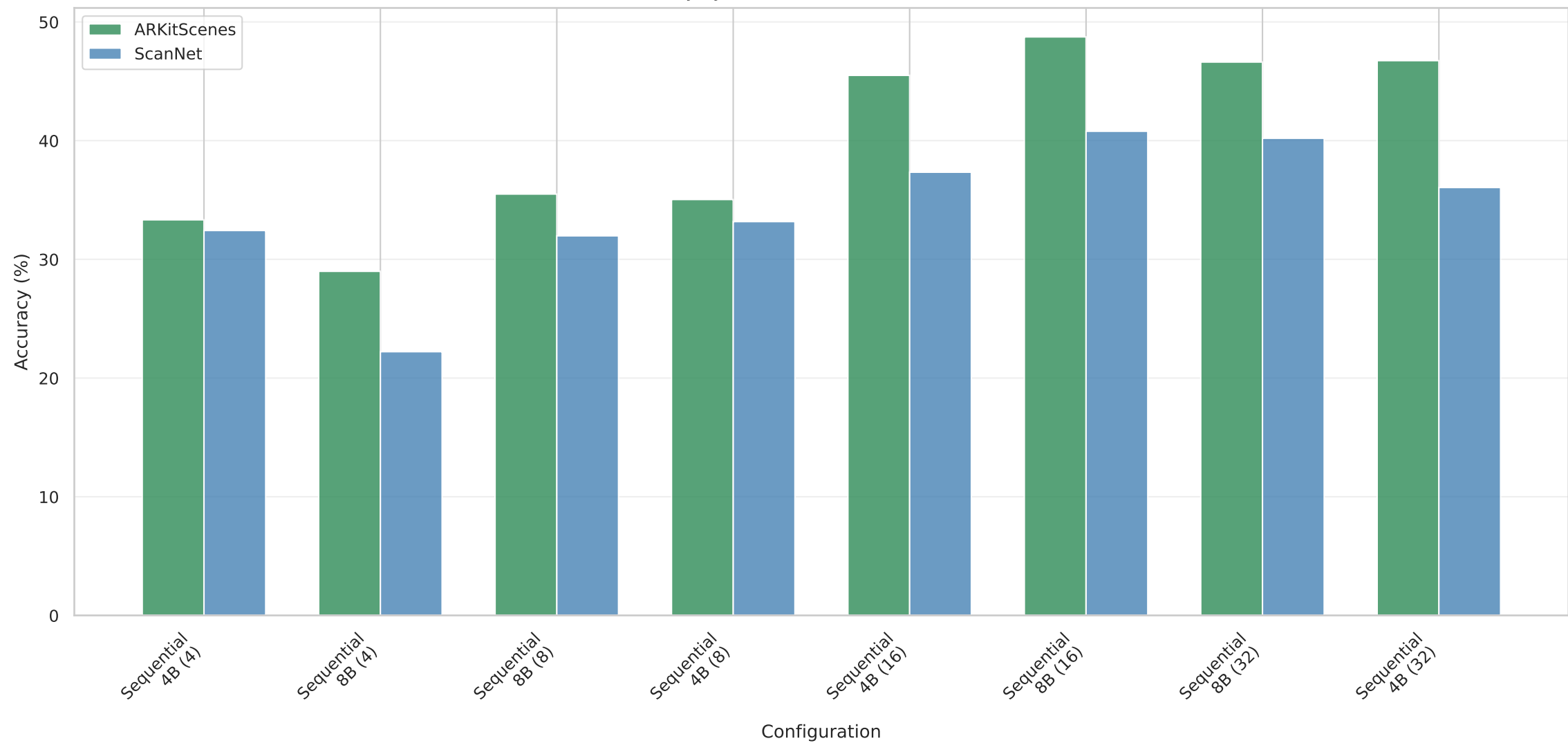
Accuracy by Dataset: ARKitScenes vs ScanNet
