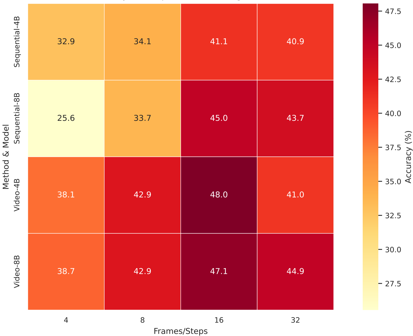
Accuracy Heatmap: Method vs Configuration
