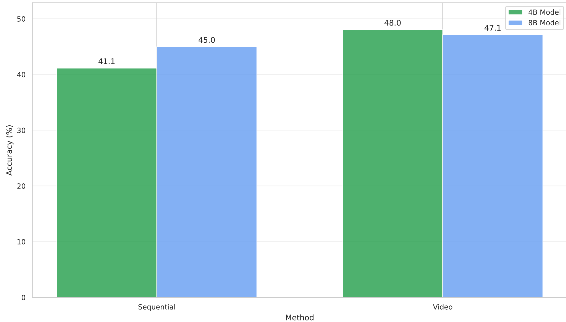
VSI-Bench: Best Accuracy by Method and Model Size
