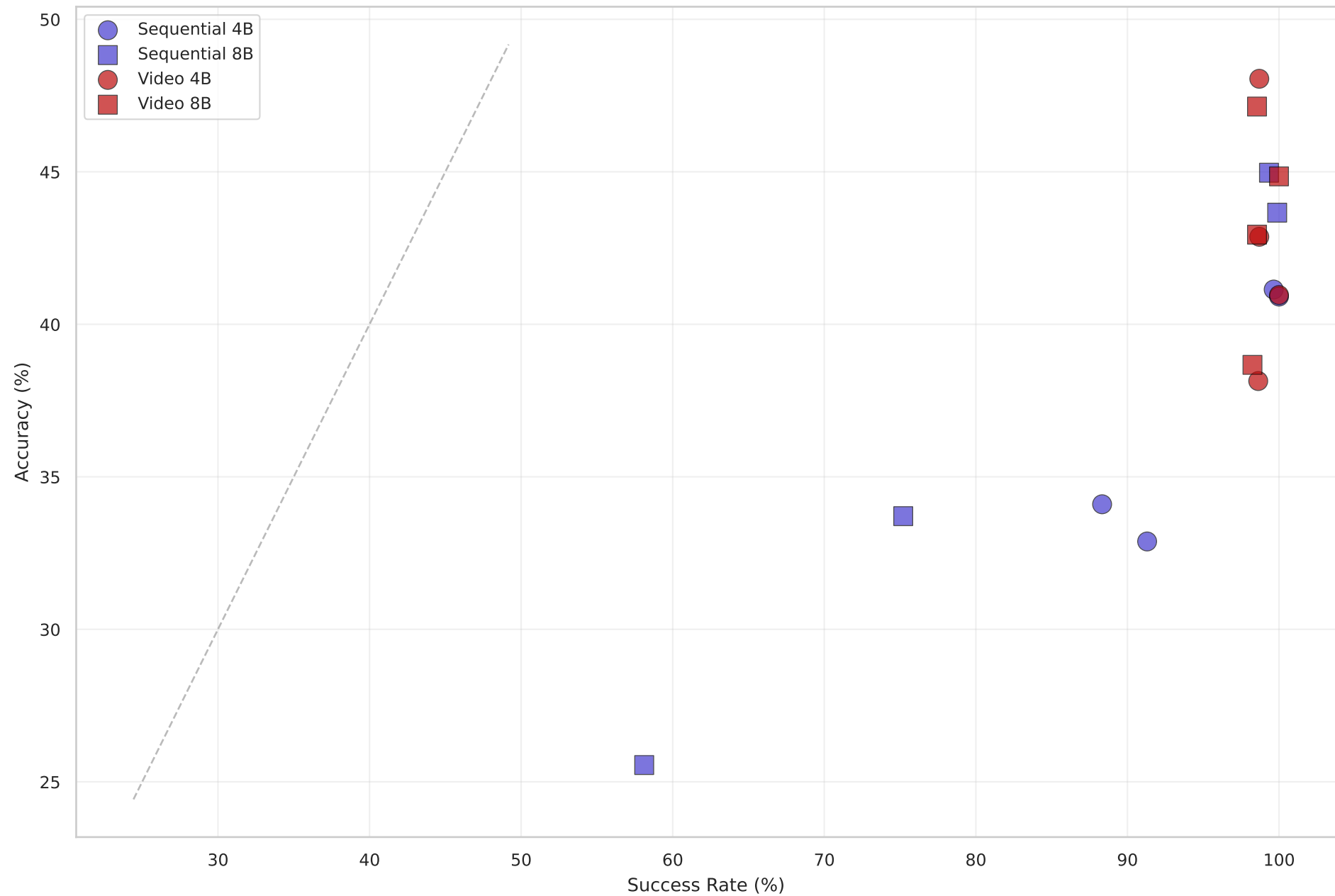
Success Rate vs Accuracy Trade-off
