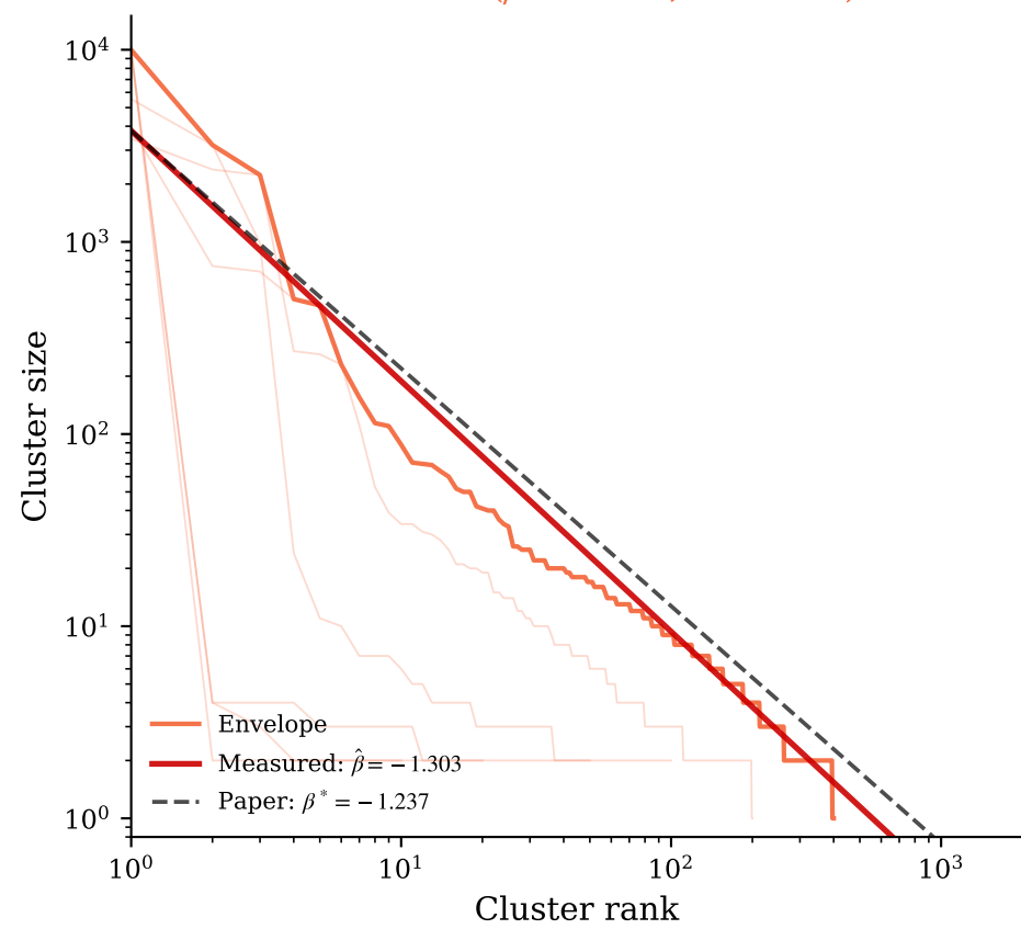
SSC-OMP ( \hat{\beta} = -1.303 , |\Delta| = 0.066 )
