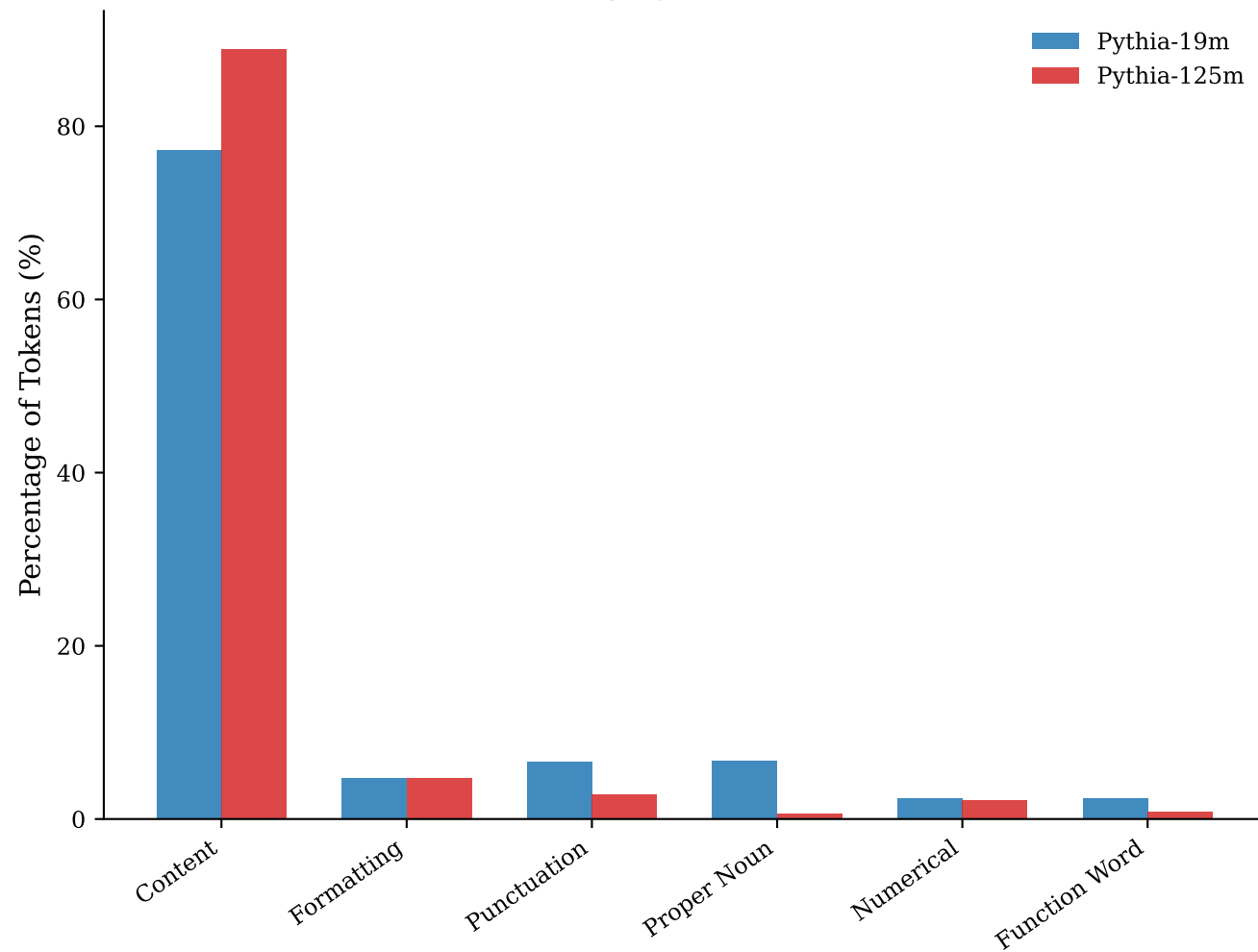
(a) Token category distribution ( k=400 )
