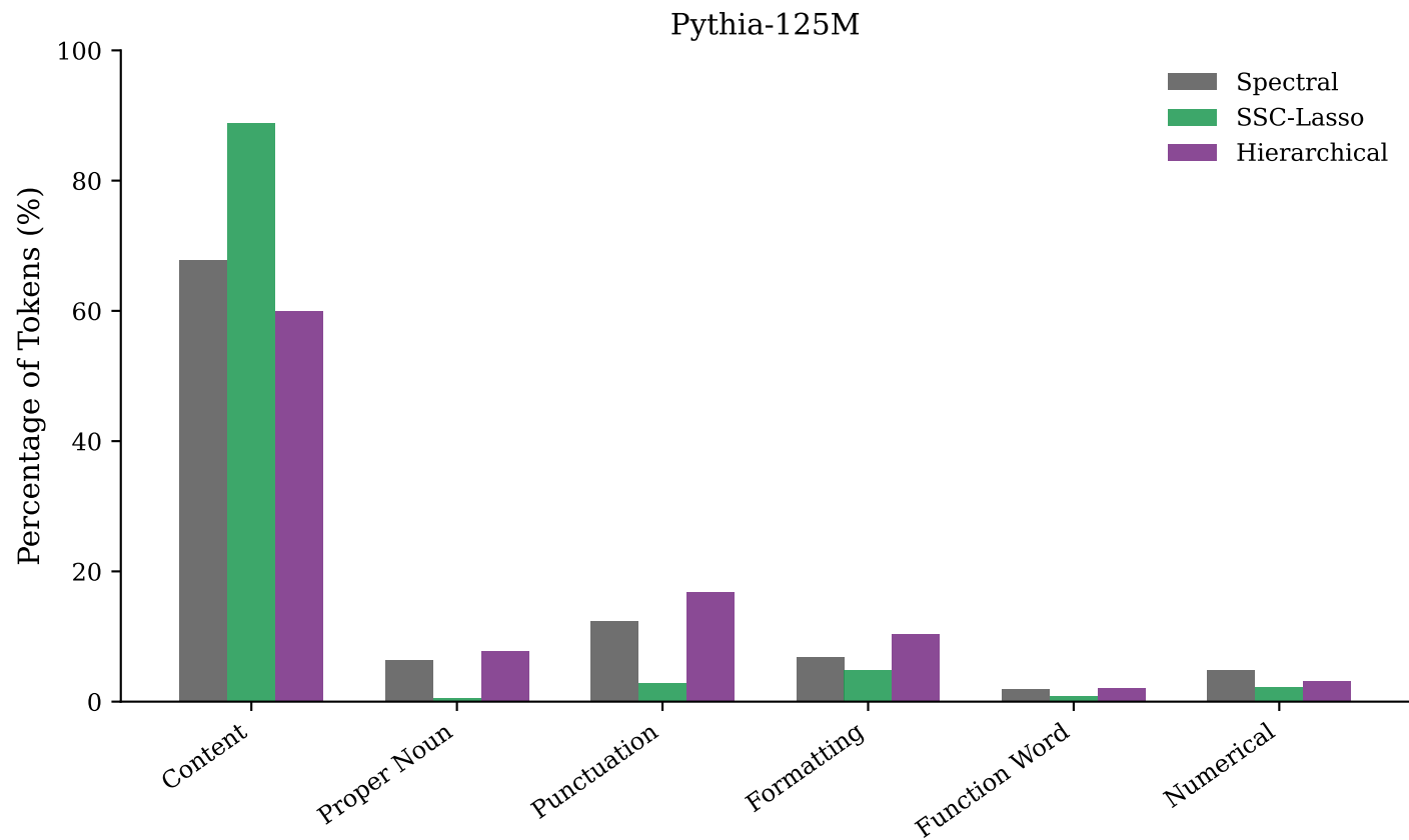
Cluster taxonomy: Spectral vs. SSC-Lasso vs. Hierarchical ( k=400 )
