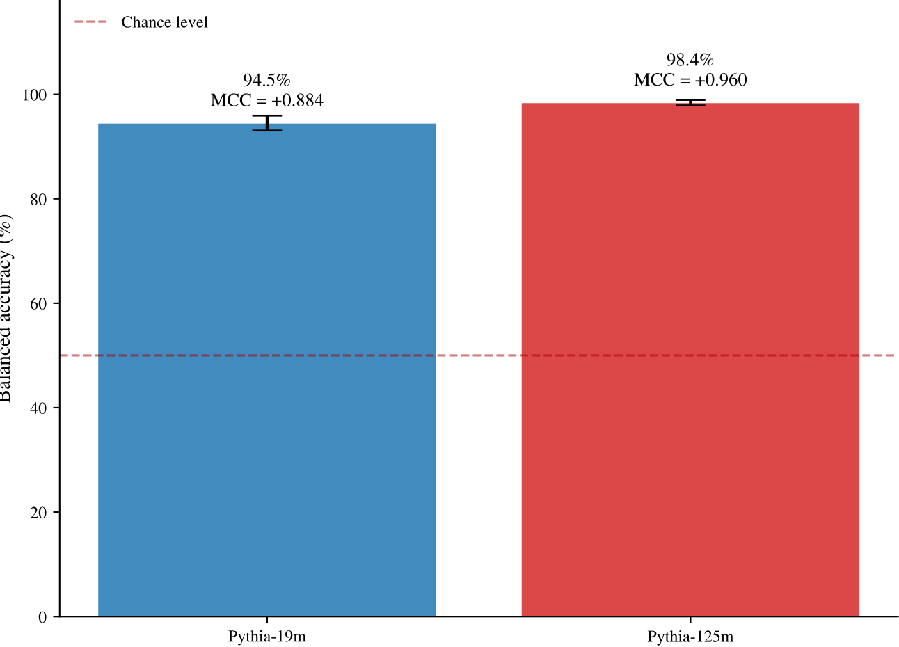
(c) Logistic regression on quanta fingerprints
