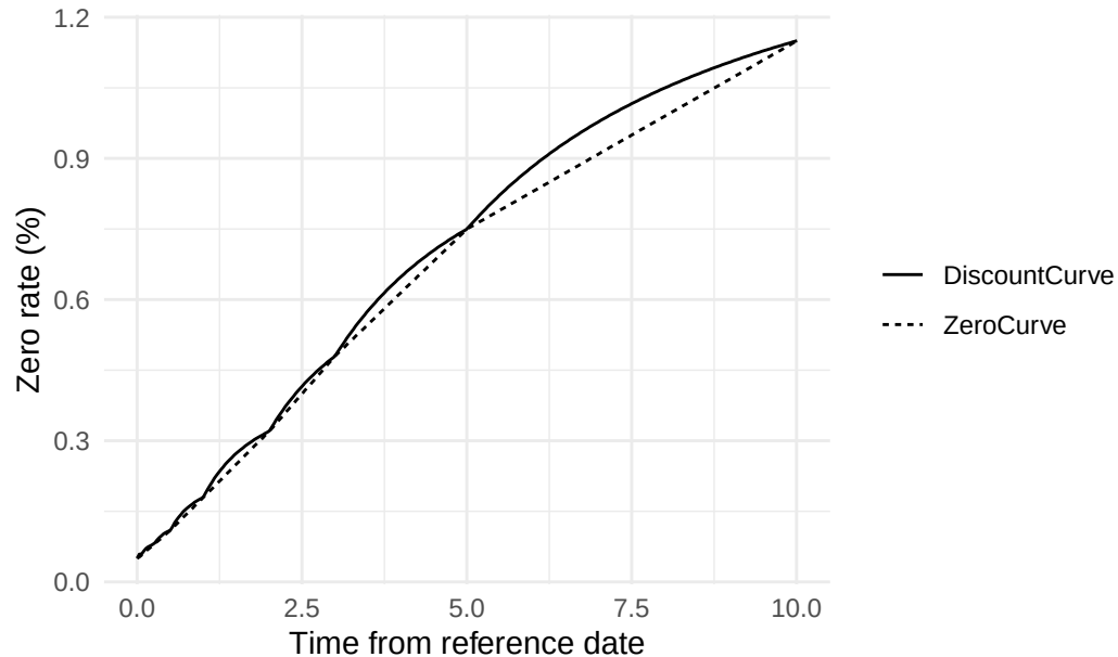
Zero rates under different interpolation targets
