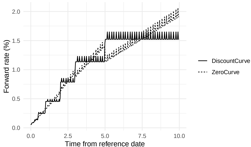
Forward rates under different interpolation targets
