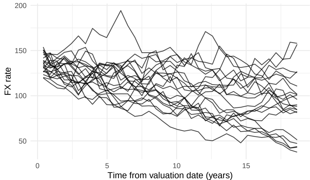
Sample FX paths for PRDC valuation
