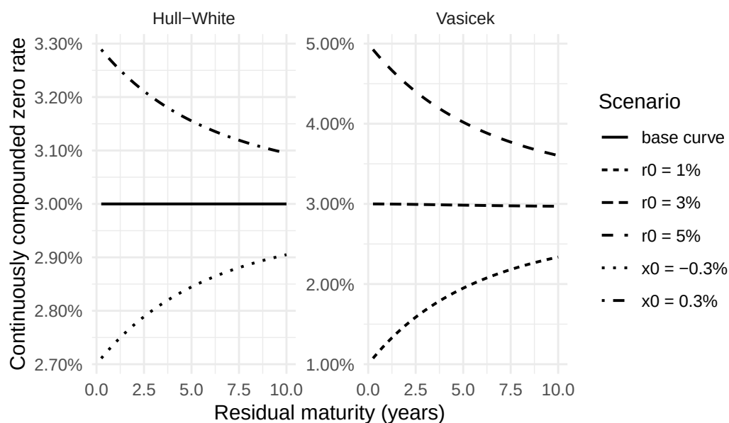
Vasicek and Hull-White zero-rate curves
