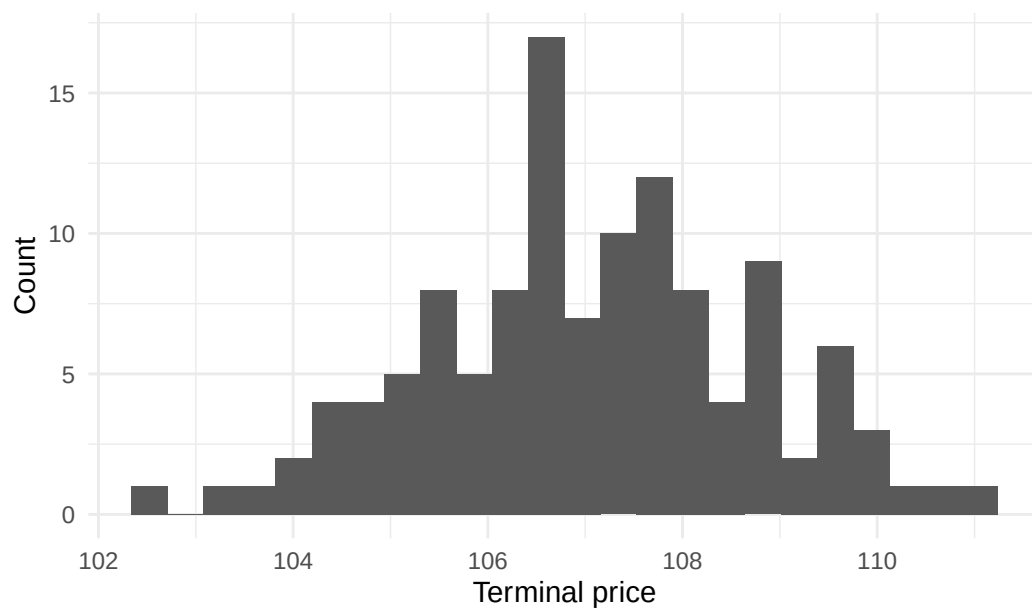
Terminal forward-price distribution
