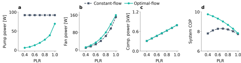
Fig. 1. Feasible GSHP part-load points: (a) pump; (b) indoor fan; (c) compressor power; (d) system COP. PLR 0.3 is infeasible.
