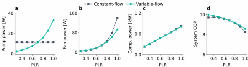
Fig. 1. Part-load performance of the GSHP under constant- and variable-flow control: (a) ground-loop pump power; (b) indoor-fan power; (c) compressor power; and (d) system COP.
