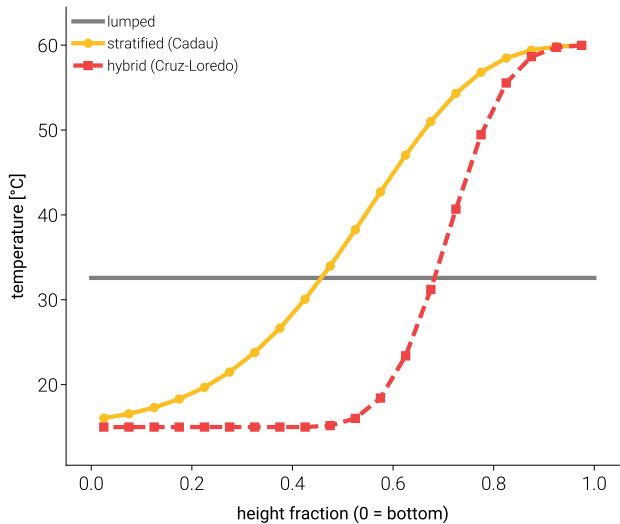
charging thermocline (N=20, front ~mid)
