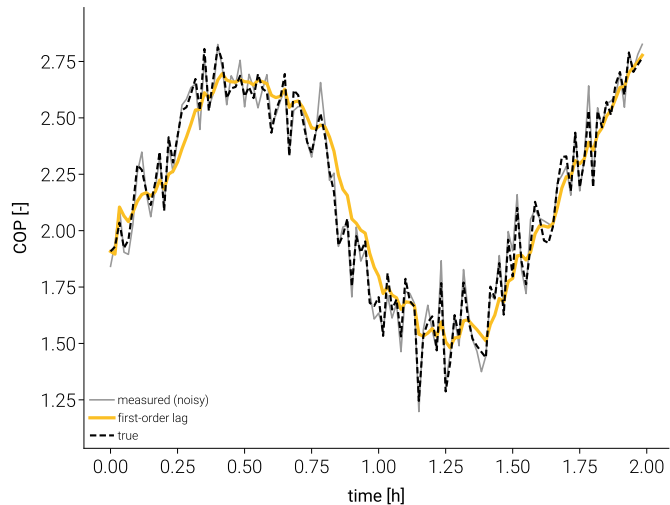
first-order lag smoothing
