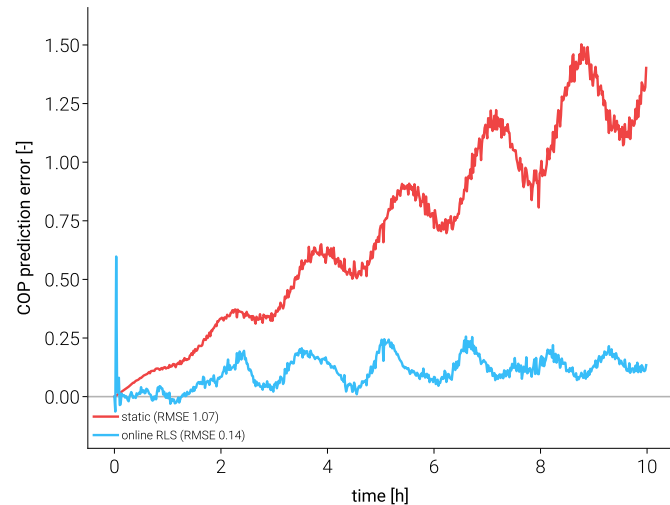
tracking a drifting cycle
