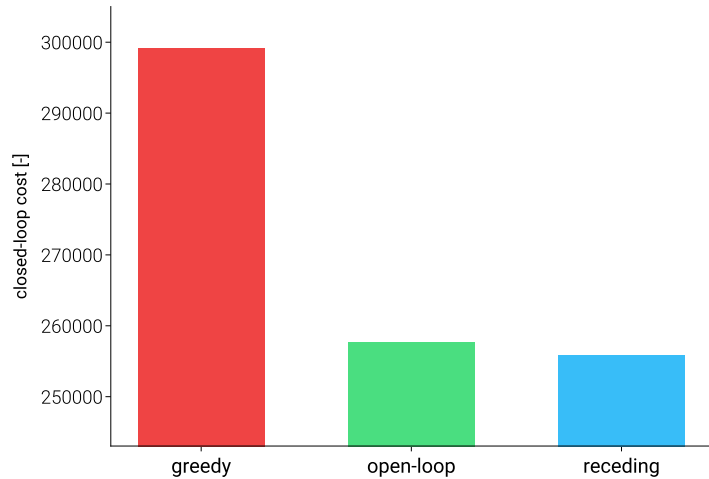
cost under model-plant mismatch
