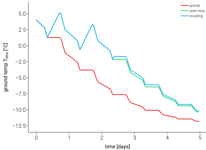
closed-loop ground (plant depletes faster than model)
