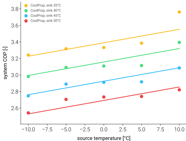
ASHP (source = outdoor air) RMSE=0.071, max|err|=0.209
