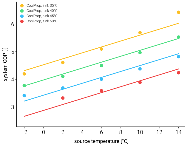
GSHP (source = ground) RMSE=0.143, max|err|=0.398
