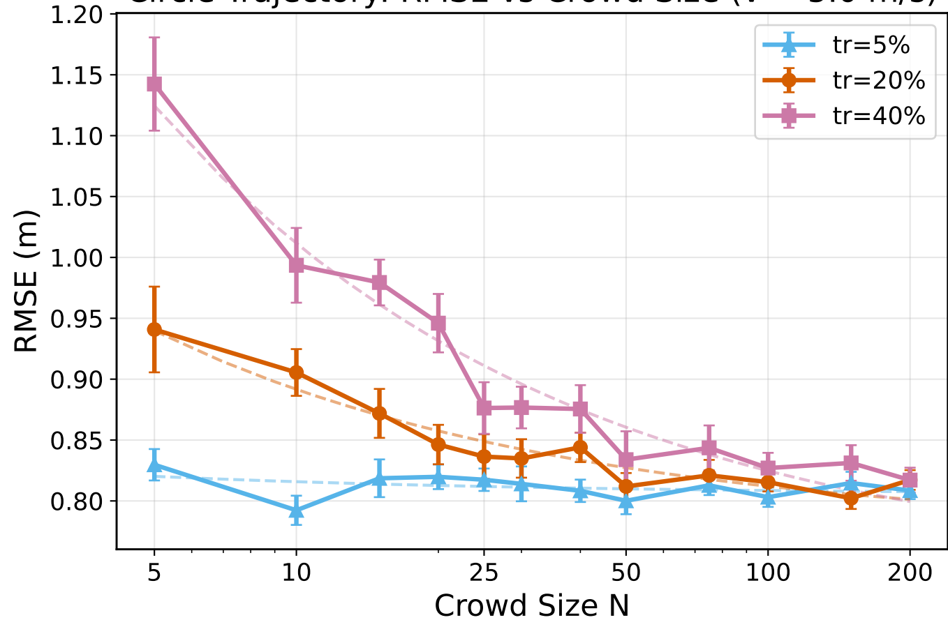
Circle Trajectory: RMSE vs Crowd Size ( v = 5.0 m/s)
