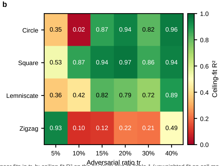
a: b from the a + b/\sqrt{N} fit (weighted least squares, 1/\text{sem}^2 ), bars 95% CI, dashed lines linear fits in tr . b: ceiling-fit R^2 on the six-level grid of Table 1 (unweighted fit on cell means, corrected data).
