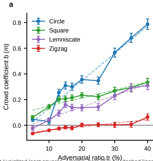
a: b from the a + b/\sqrt{N} fit (weighted least squares, 1/\text{sem}^2 ), bars 95% CI, dashed lines linear fits in tr . b: ceiling-fit R^2 on the six-level grid of Table 1 (unweighted fit on cell means, corrected data).
