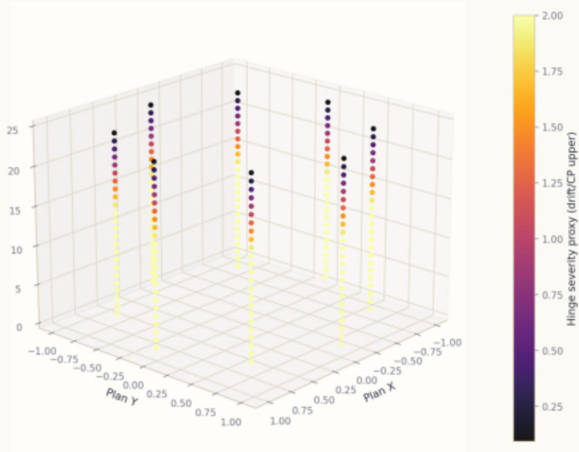
3D Plastic-Hinge Proxy (opstool_606m_megatall_model-00001)
